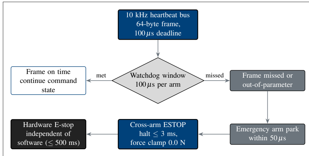
Figure 14. Heartbeat, watchdog, and E-stop architecture. A 10 kHz heartbeat bus with a 100\mu\text{s} per arm watchdog continues the command state on an on-time frame; a missed frame parks the arm within 50\mu\text{s} and escalates to a cross-arm E-stop that halts the platform in \leq 3 ms at a 0.0 N force clamp, backed by a software independent hardware E-stop meeting the §312.404 \leq 500 ms requirement.
